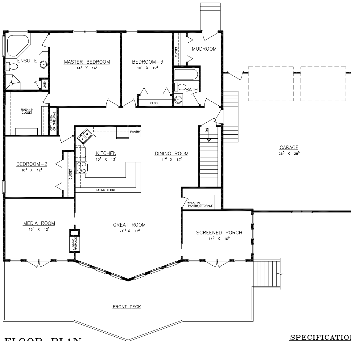
FLOOR PLAN
